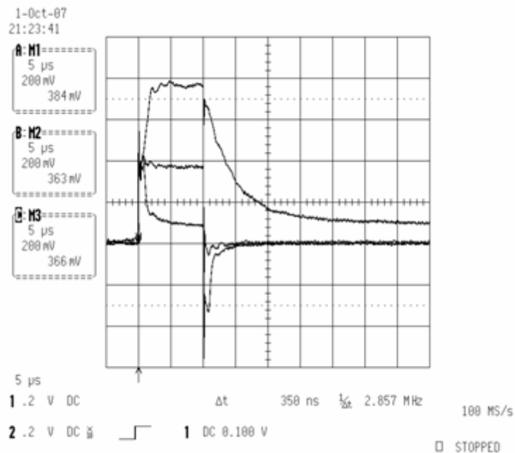
Typical John Bedini SG Bifilar Motor Coil
